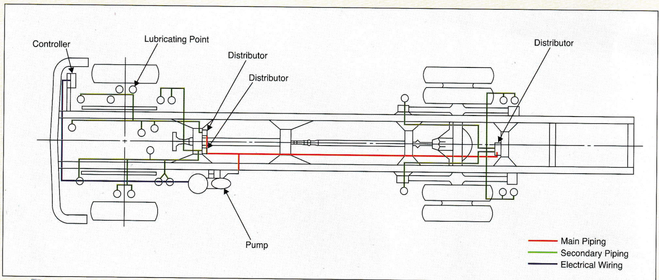
Equipment Lay-out Drawing
